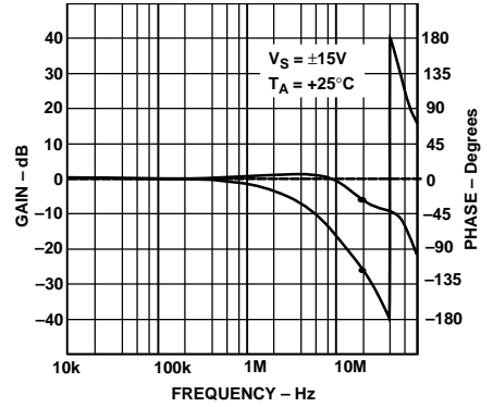
Closed-Loop Gain and Phase, A_V = +1
