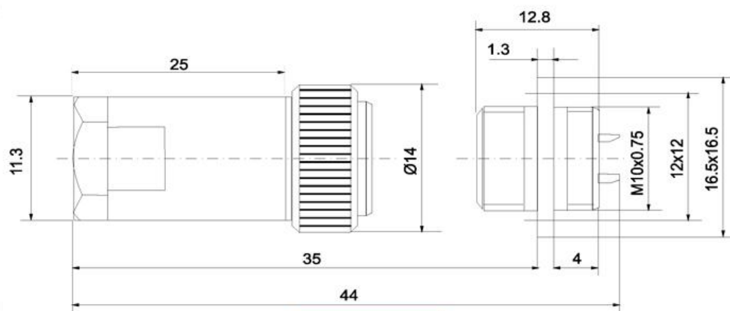
SZC-CONNECTOR
